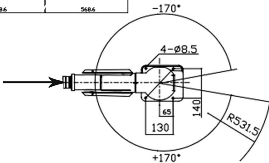
底座安装图 Base installation drawing
