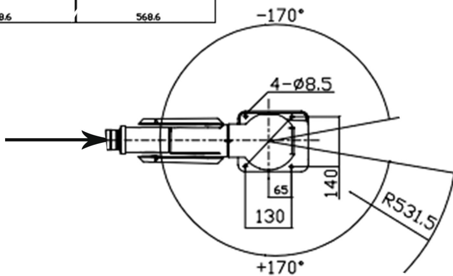
Base installation drawing
