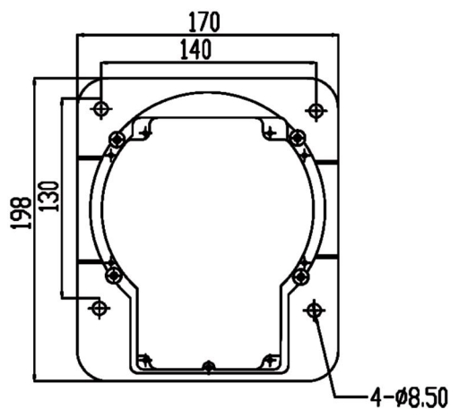
Base installation drawing
