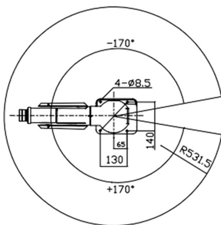
Flange drawing
